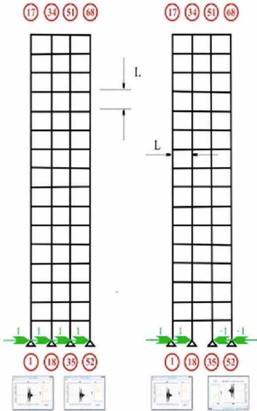
Fig. 4. Example building Calculated by SAP 2000 [12] and MatLab [13]
