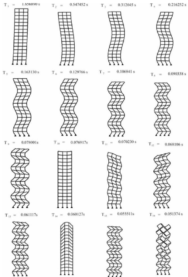
Fig. 5. Eigenmodes and Eigenperiods. Calculated by SAP 2000 [12] and MatLab [13]
