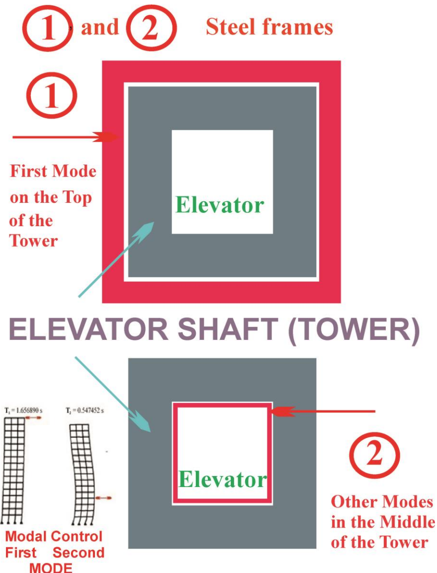
Fig. 7. Location of the inertial motors for the first and second modes of vibration (Fig. 2) for the example building of Figure 1. Compensating the earthquake (wind) dynamic effects with inertial motors in the higher modes (greater than 1) is associated with significant technical difficulties, affecting the final result insignificantly (less than 10%). It is recommended to offset only the first form.
