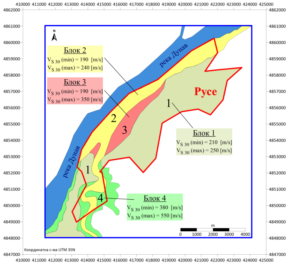
Fig. 2. Map of Vs 30 for Russe
