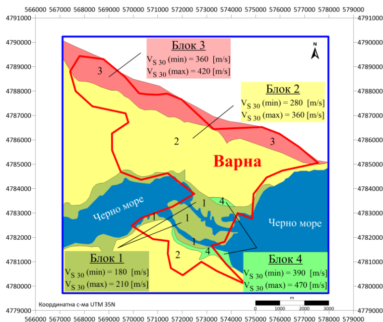
Fig.1. Map of V_s_{30} for Varna
