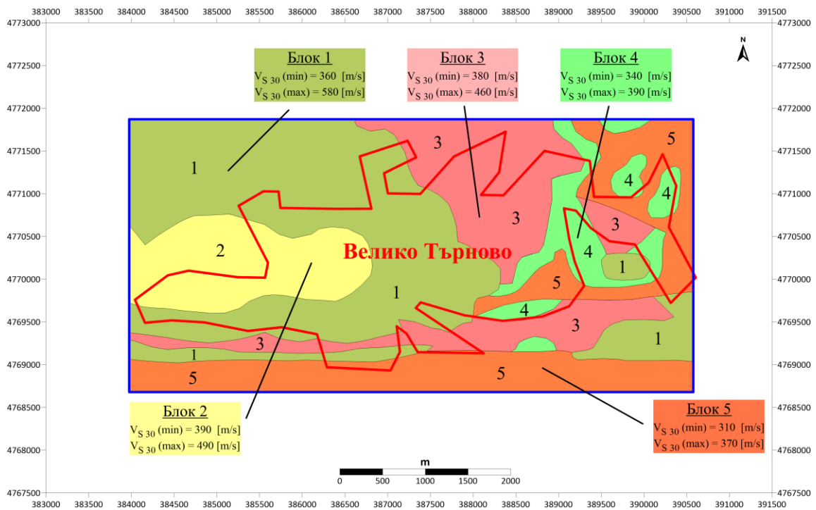
Fig. 3. Map of Vs 30 for Veliko Tarnovoe
