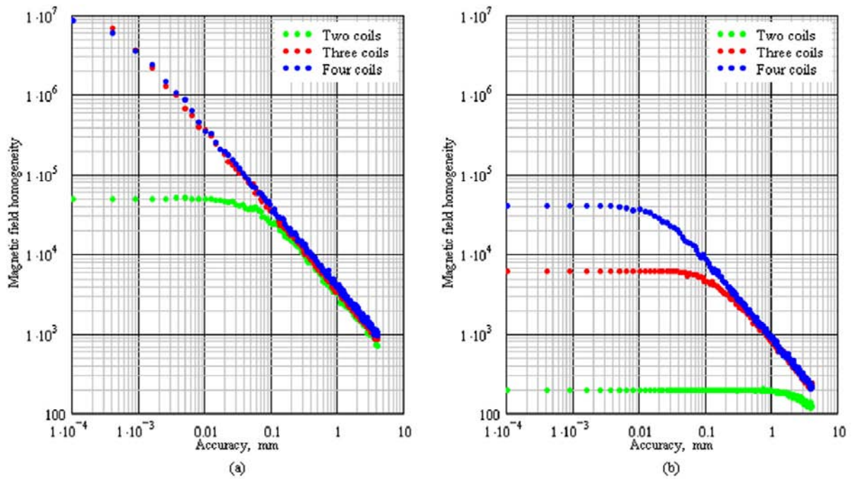
Fig. 2. Magnetic field homogeneity as a function of the mechanical accuracy in the case of square coils with side length 500 mm, in the central cubic zone with size 25 mm (a) and 100 mm (b).
