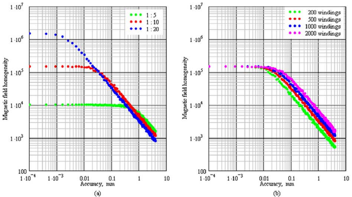
Fig. 3. Magnetic field homogeneity as a function of the mechanical accuracy in the case of circular solenoids with 1000 windings of 500 mm in diameter and different diameter-to-the-length ratio (a) and solenoids with diameter 500 mm, diameter-to-the-length ratio 1:10 and different number of windings (b). Zone size is 100 mm.
