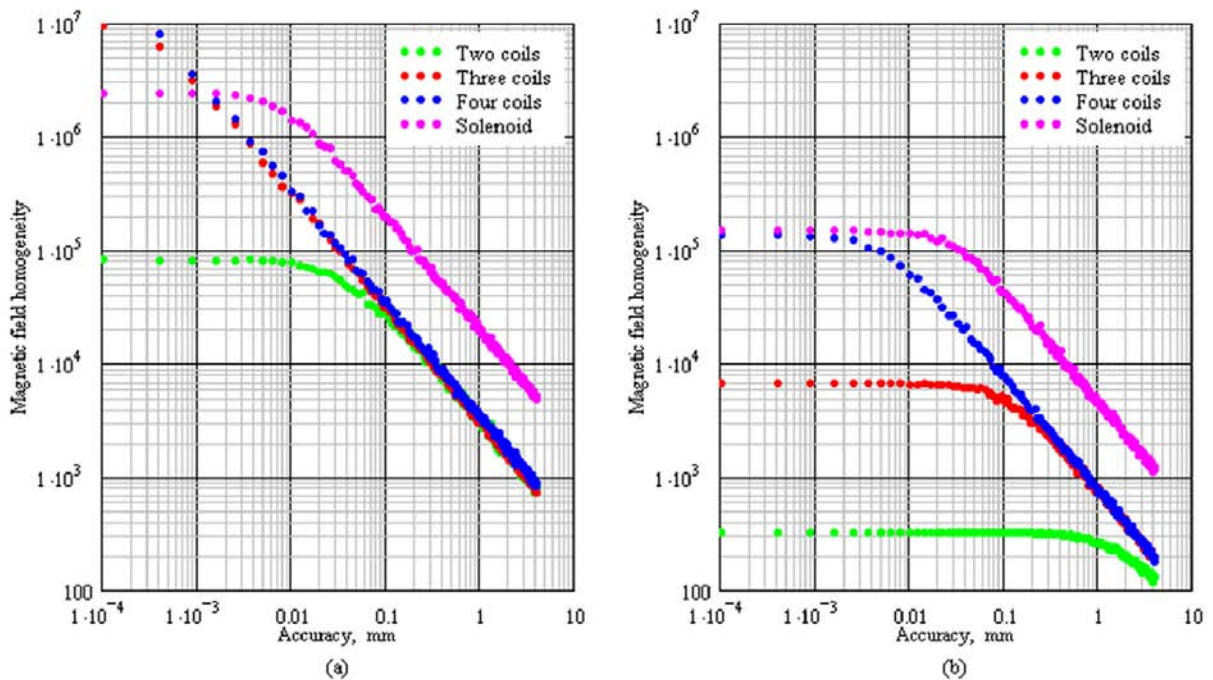
Fig. 1. Magnetic field homogeneity in the central cylindrical zone as a function of the mechanical accuracy in the case of circular coils with 500 mm diameter and 1000 windings solenoid with diameter-to-the-length ratio of 1:10 and 500 mm diameter. Zone size is 25 mm (a) and 100 mm (b) respectively.
